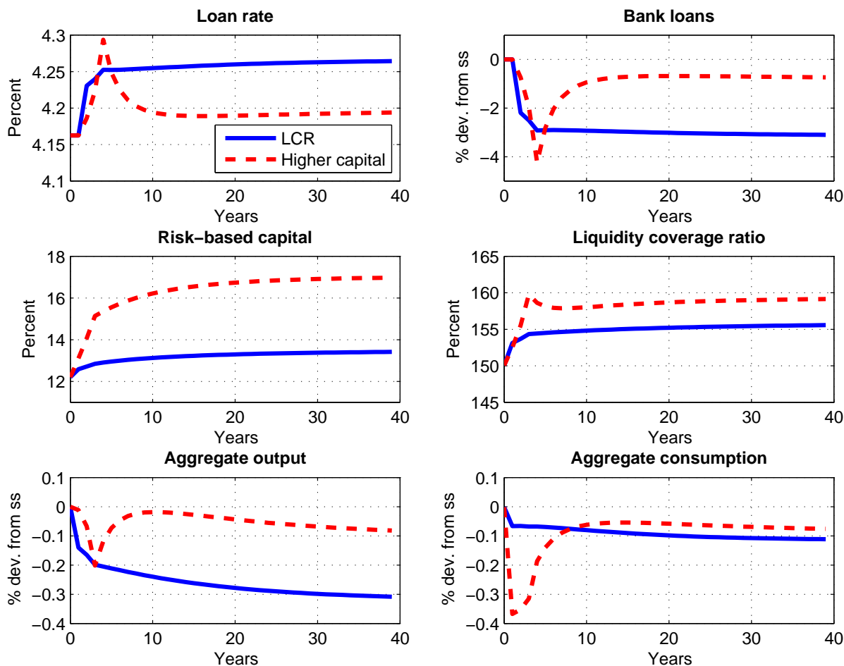
Figure 5: Comparison of Introducing Liquidity Requirements with Increasing Capital Requirements
