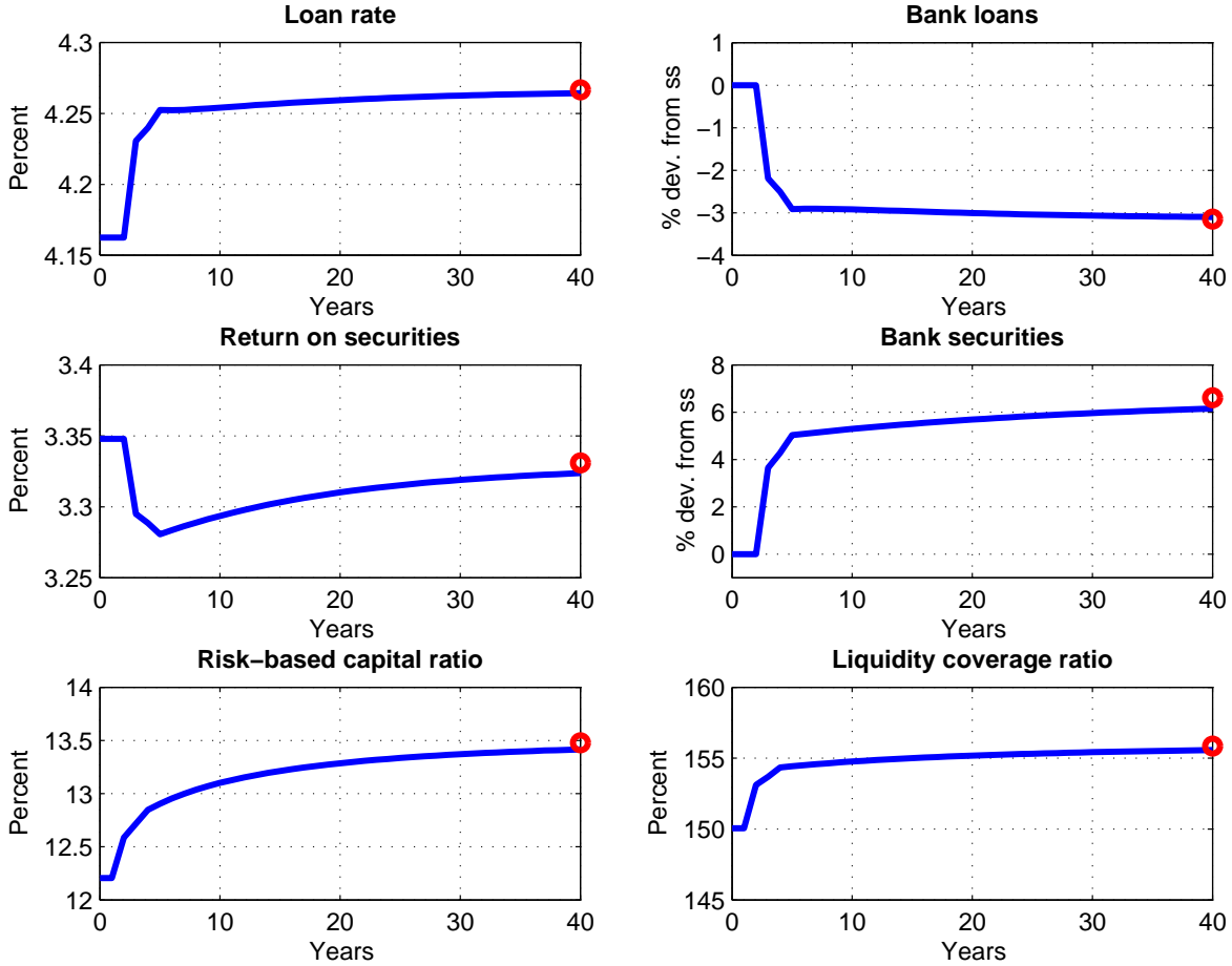
Figure 3: Introduction of Liquidity Requirements
