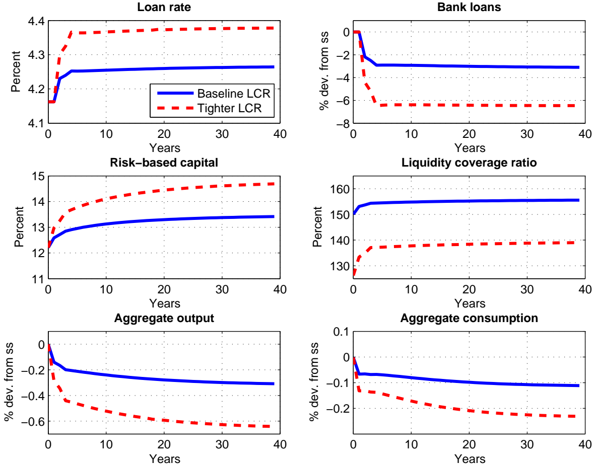
Figure 6: Introducing More Stringent Liquidity Requirements
