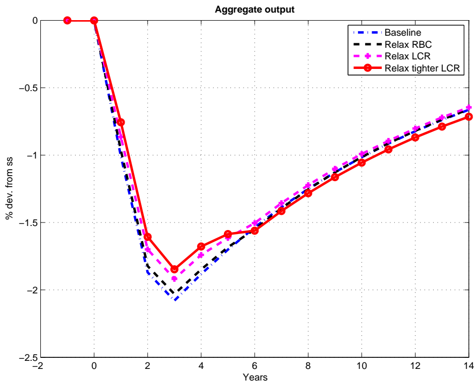
Figure 7: Aggregate Response of Output to a Wealth Shock
