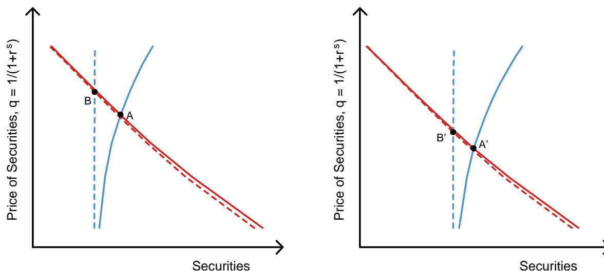
Figure 2: The Effects of an Increase in the Supply of Safe Assets
