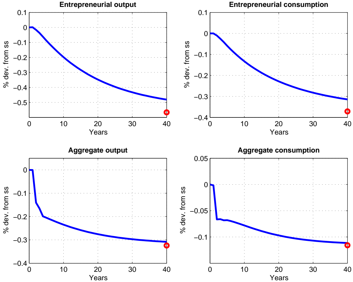
Figure 4: Introduction of Liquidity Requirements
